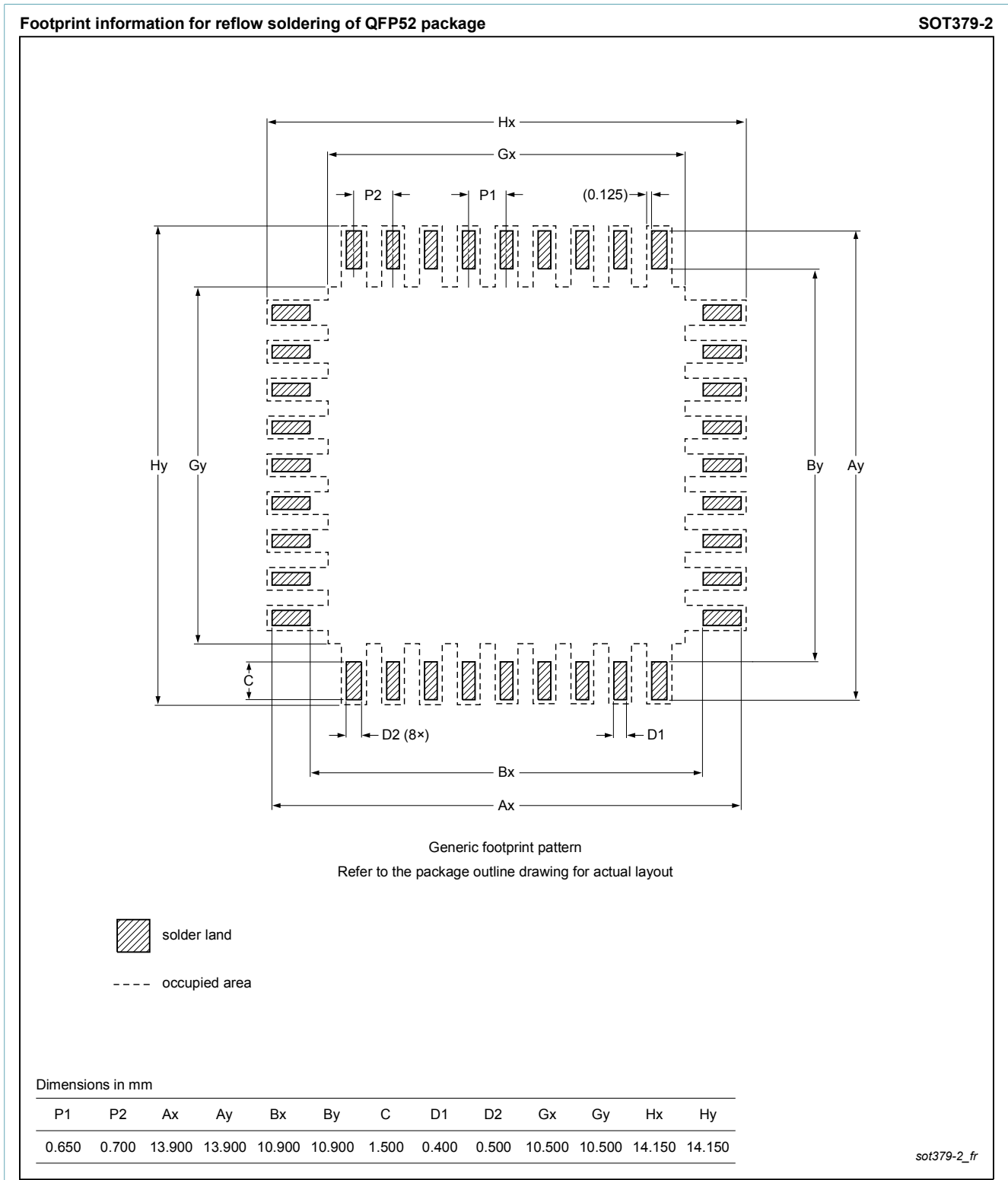
Fig. 2. Reflow soldering footprint for QFP52 (SOT379-2)
