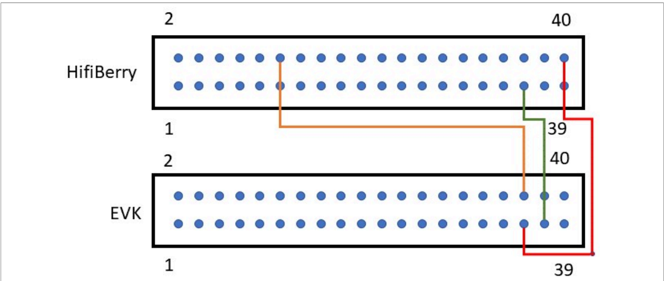
Figure 9. Transposer (Top View)
