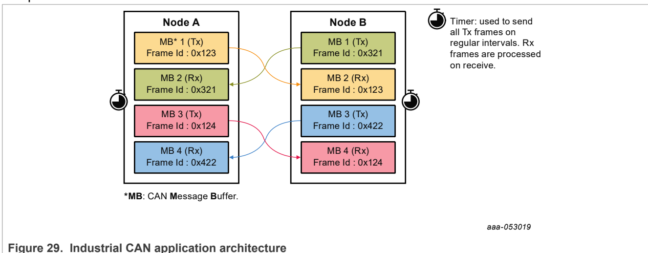
Figure 29. Industrial CAN application architecture
