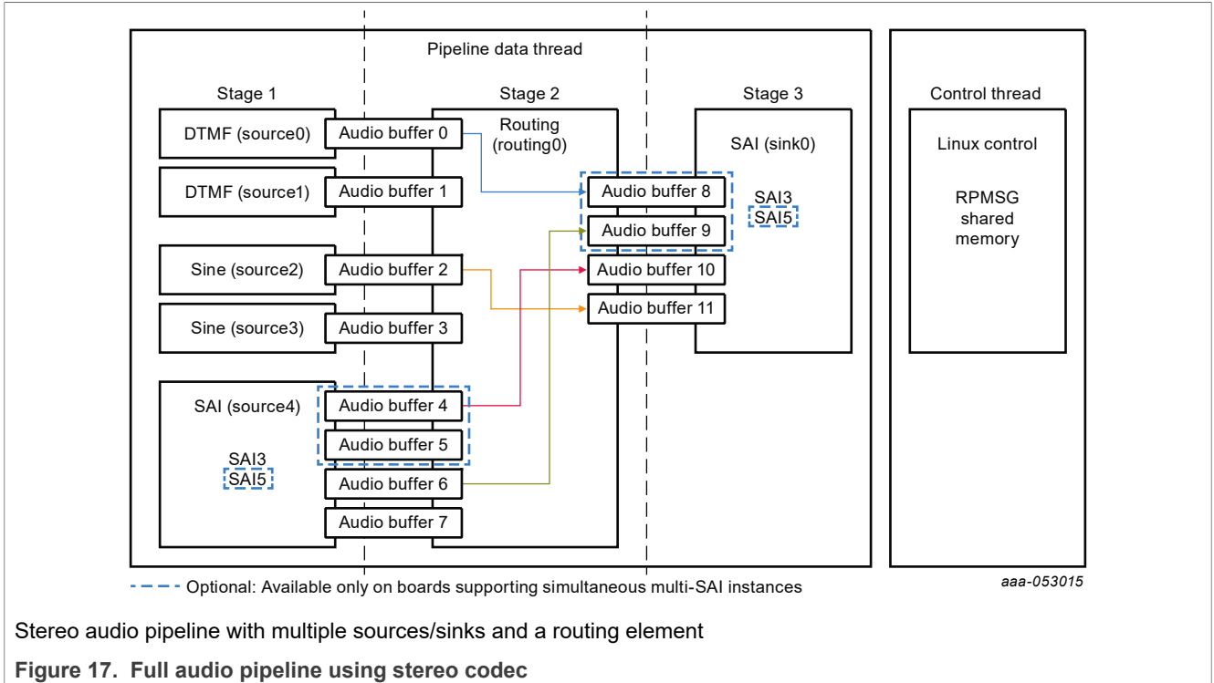
Figure 17. Full audio pipeline using stereo codec
