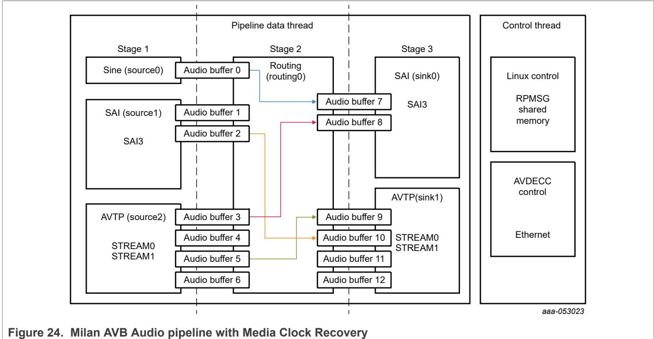
Figure 24. Milan AVB Audio pipeline with Media Clock Recovery
