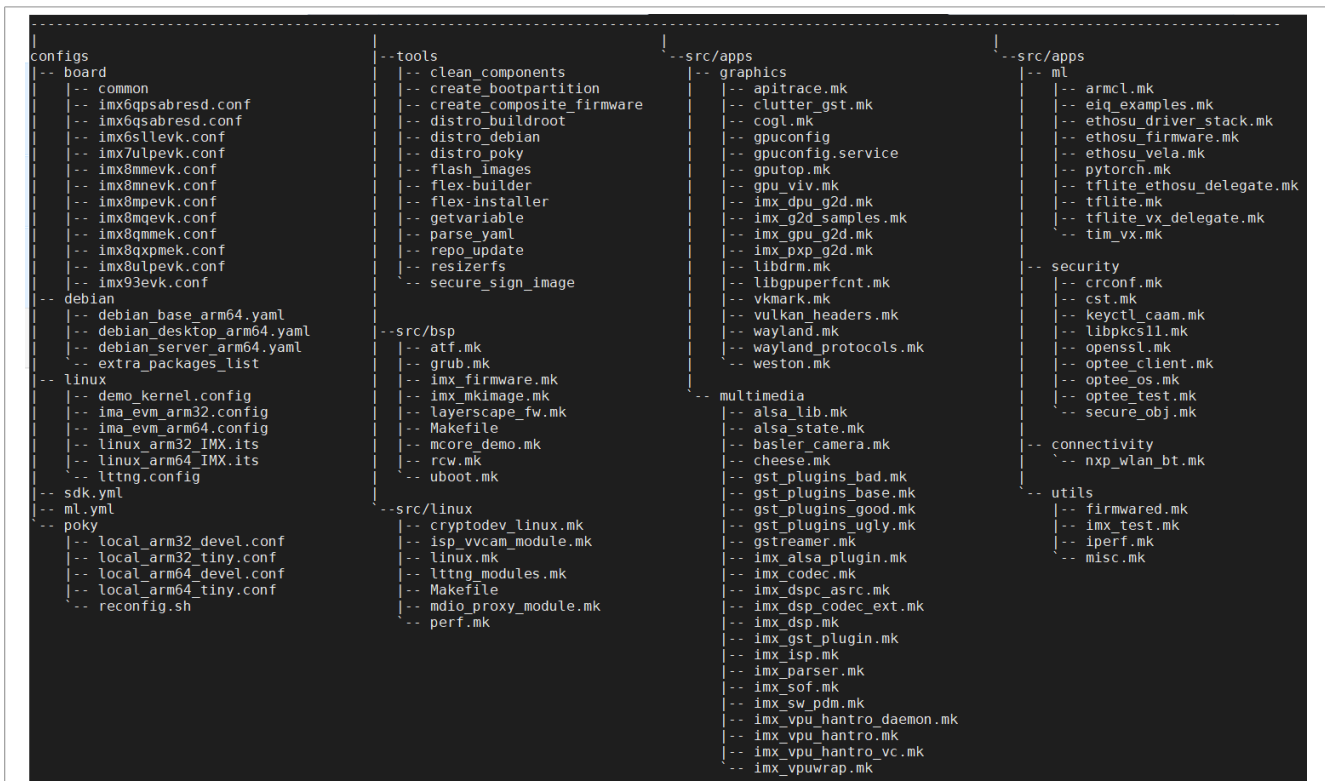
Figure 9. Flexbuild repository structure
