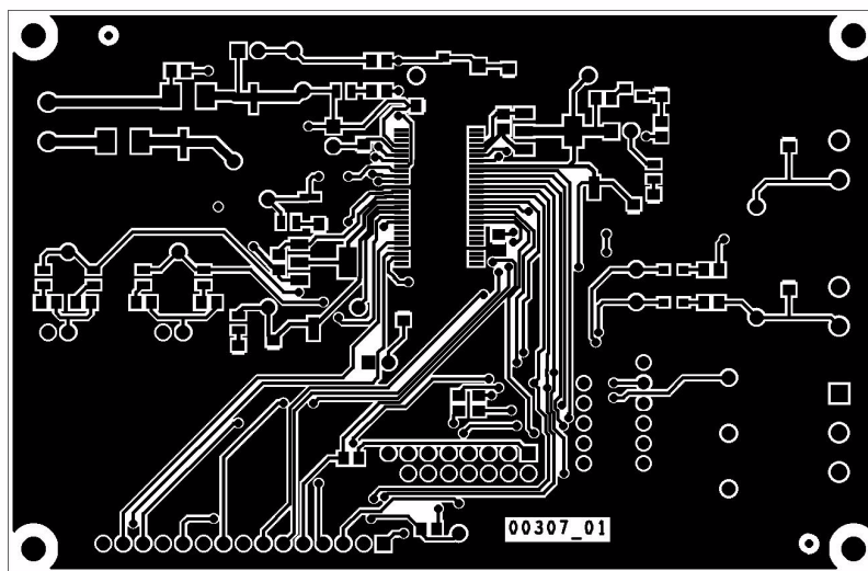
Figure 12. Top Side Layer
