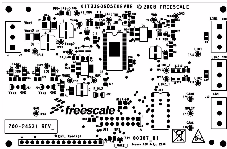
Figure 11. Assembly Drawing
