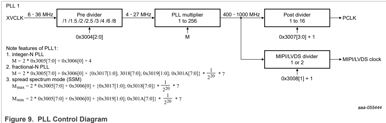
Figure 9. PLL Control Diagram
