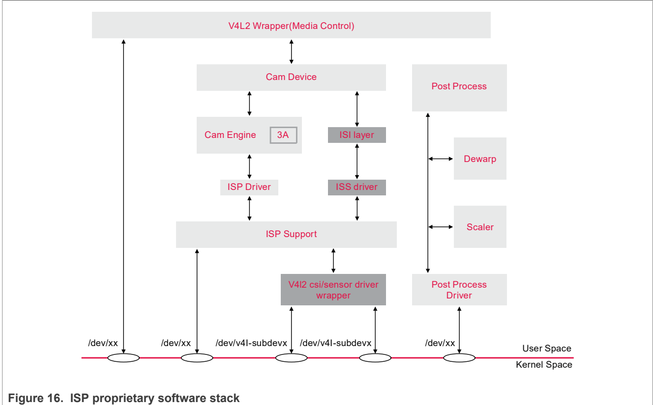
Figure 16. ISP proprietary software stack
