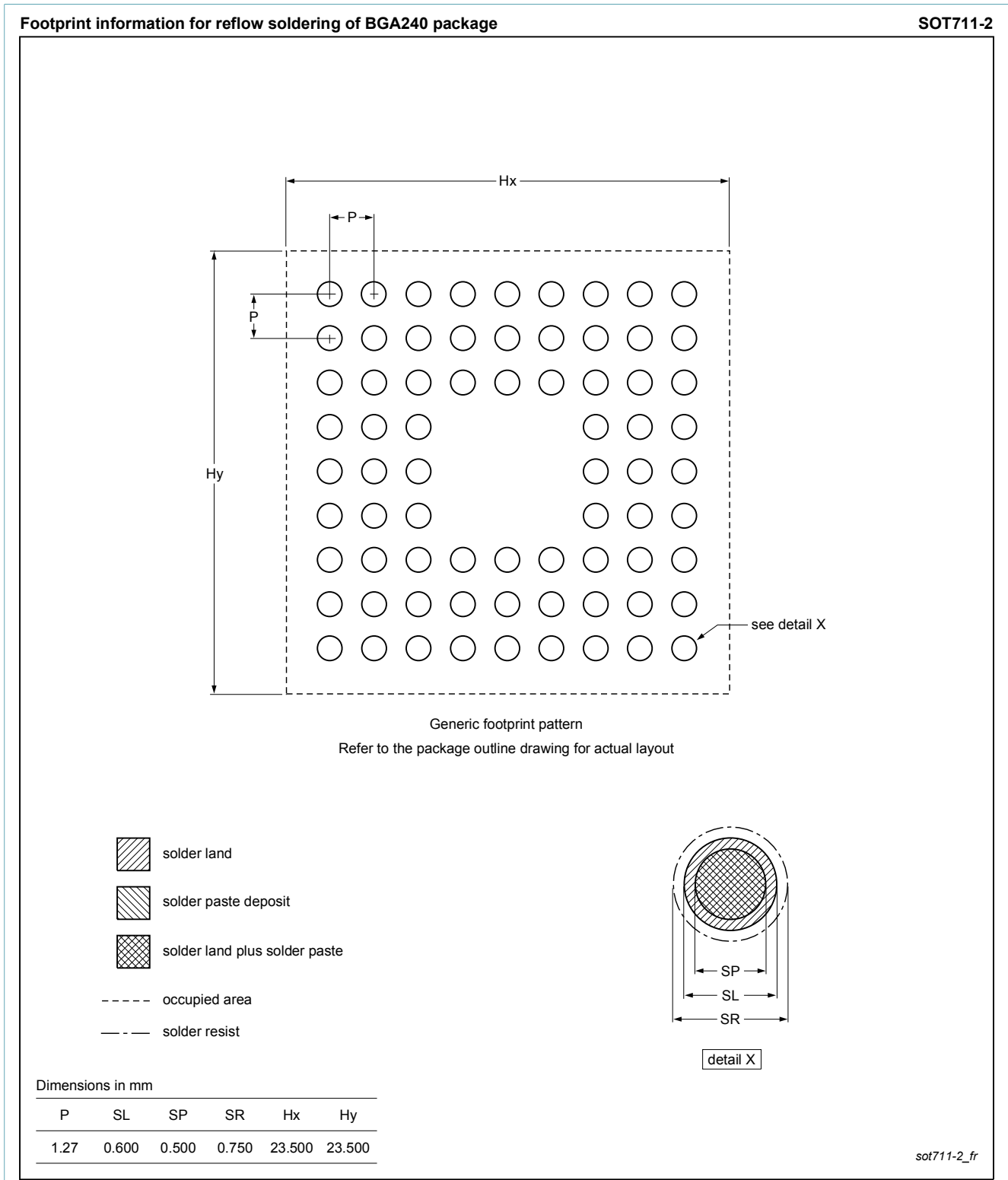
Fig. 2. Reflow soldering footprint for BGA240 (SOT711-2)
