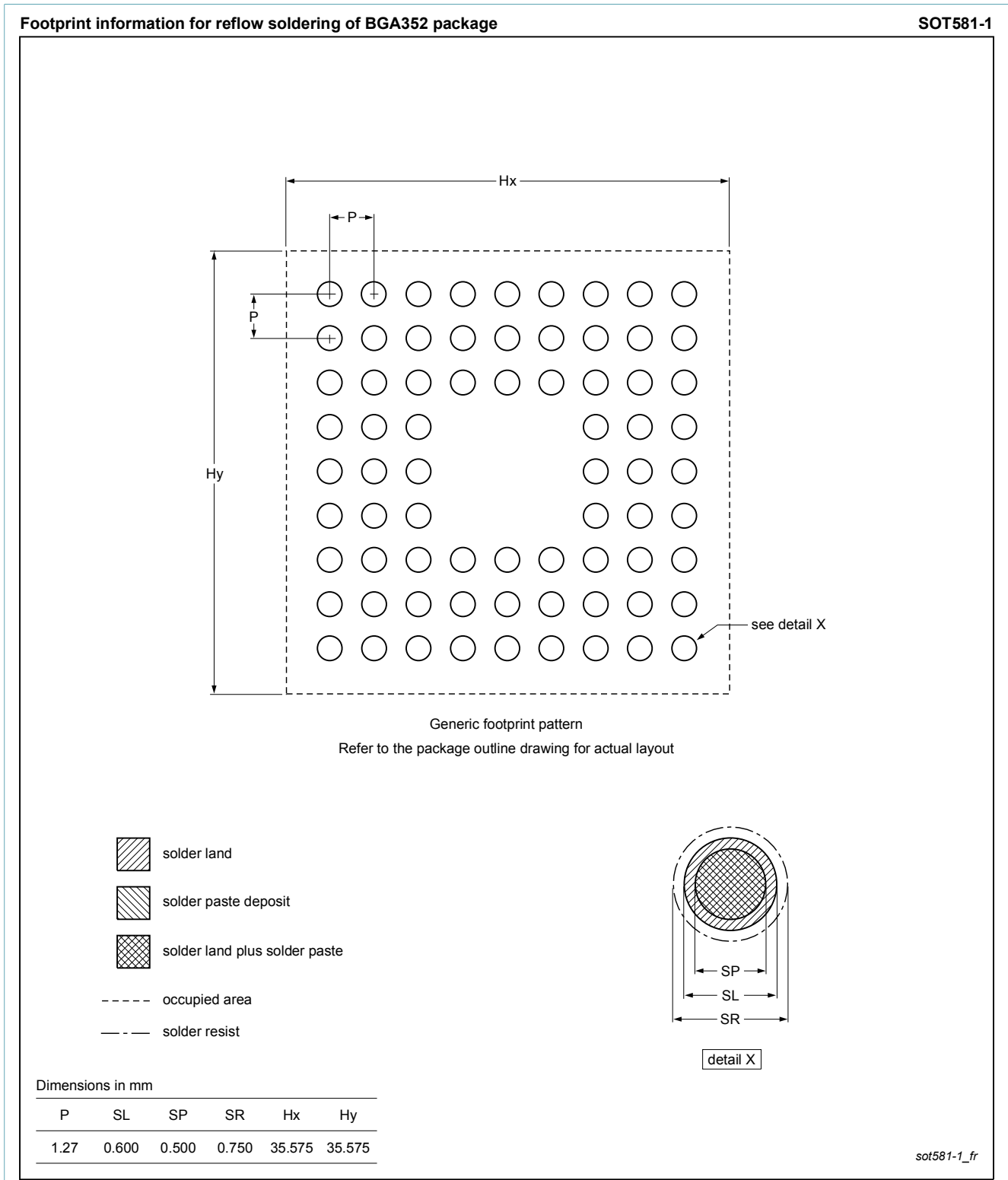
Fig. 2. Reflow soldering footprint for BGA352 (SOT581-1)
