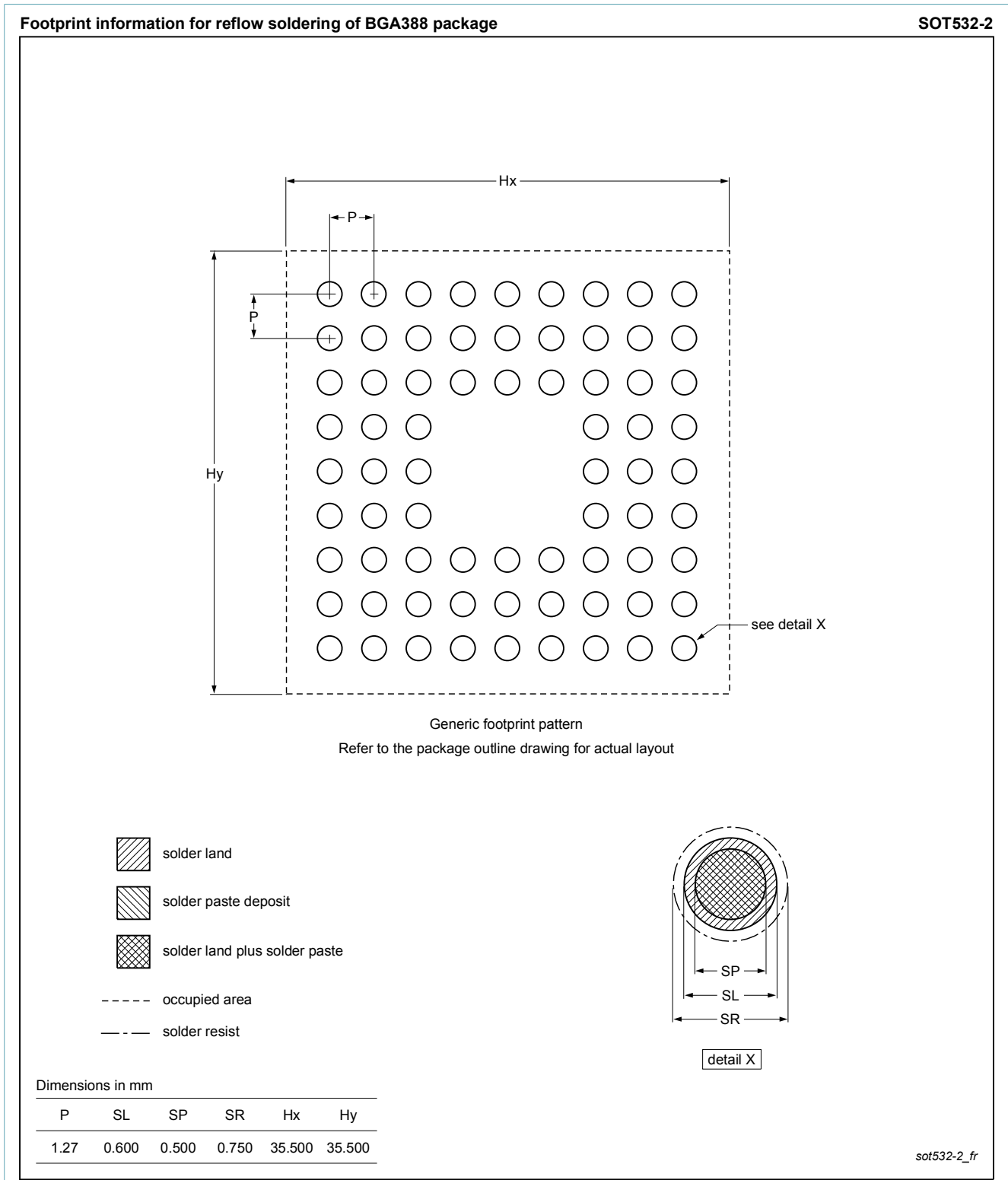
Fig. 2. Reflow soldering footprint for BGA388 (SOT532-2)
