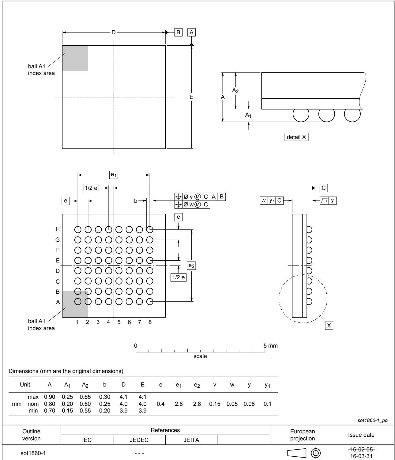
Fig. 1. Package outline VFBGA (SOT1860-1)
