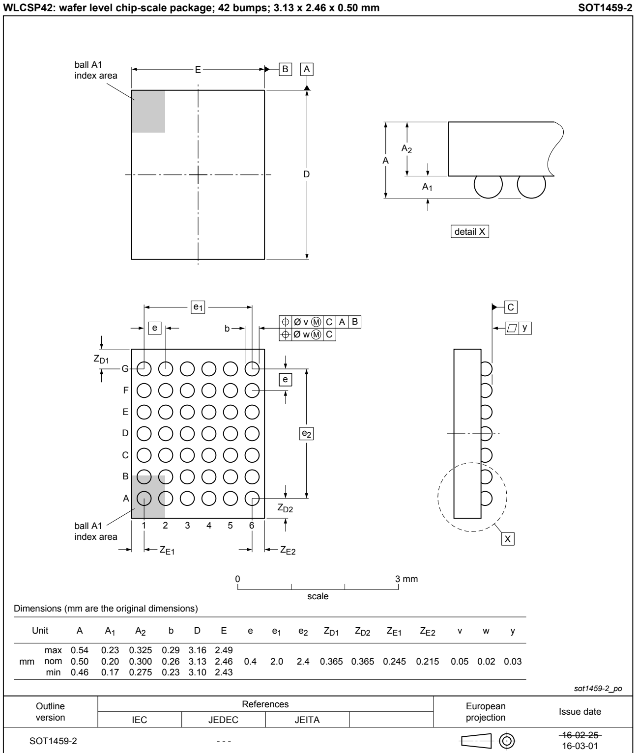
Fig. 1. Package outline WLCSP42 (SOT1459-2)
