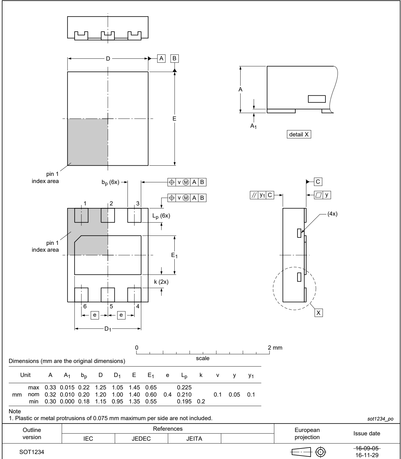
Fig. 1. Package outline HX2SON6 (SOT1234)
