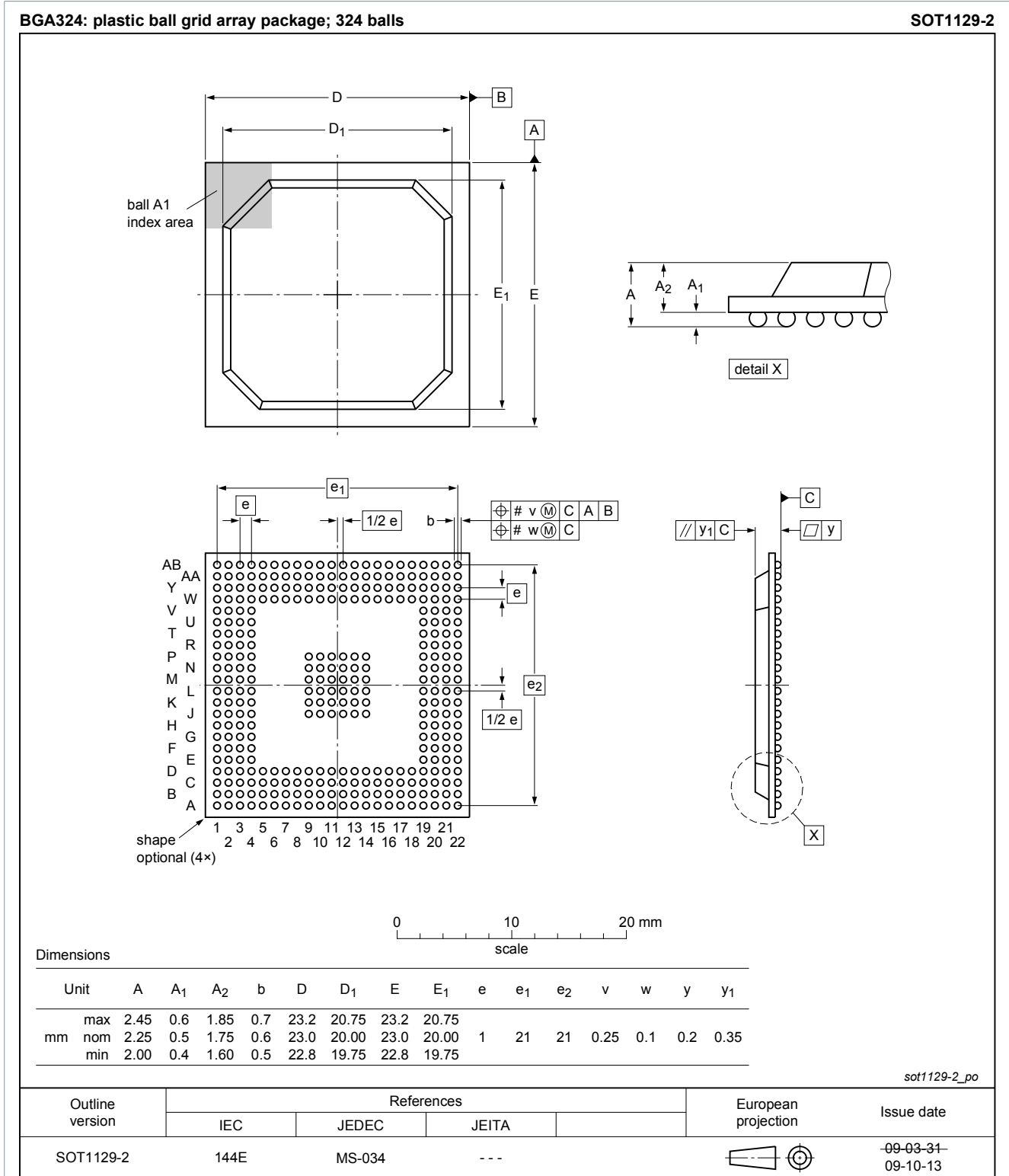
Fig. 1. Package outline BGA324 (SOT1129-2)
