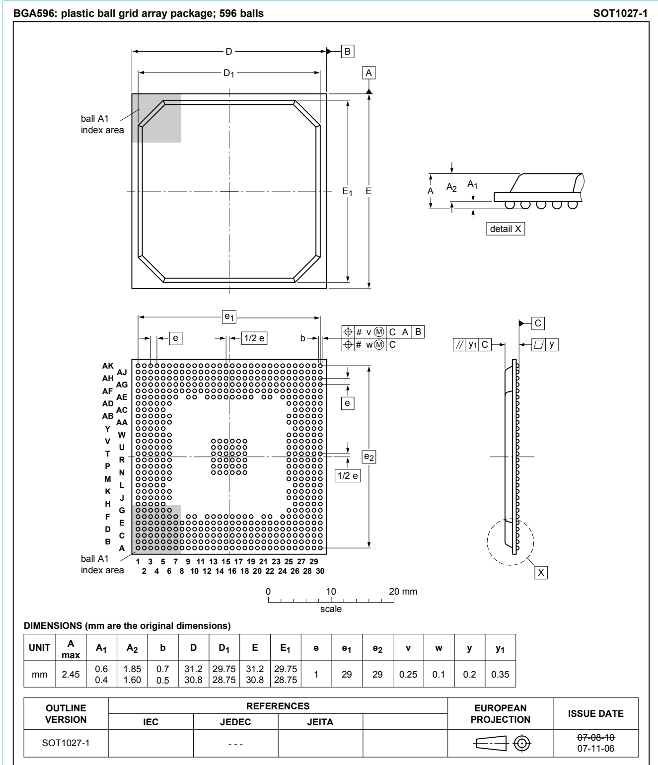
Fig. 1. Package outline BGA596 (SOT1027-1)
