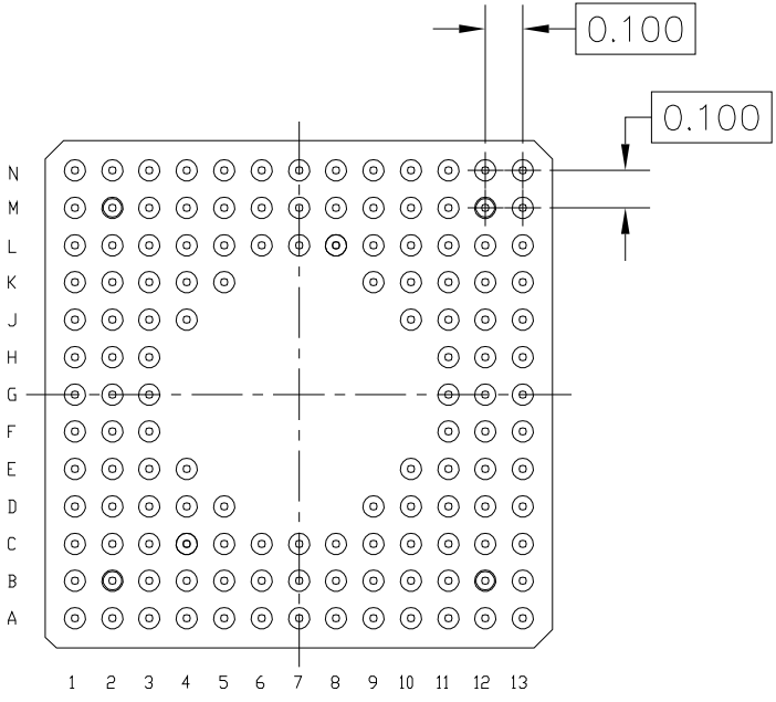
VIEW M-M
