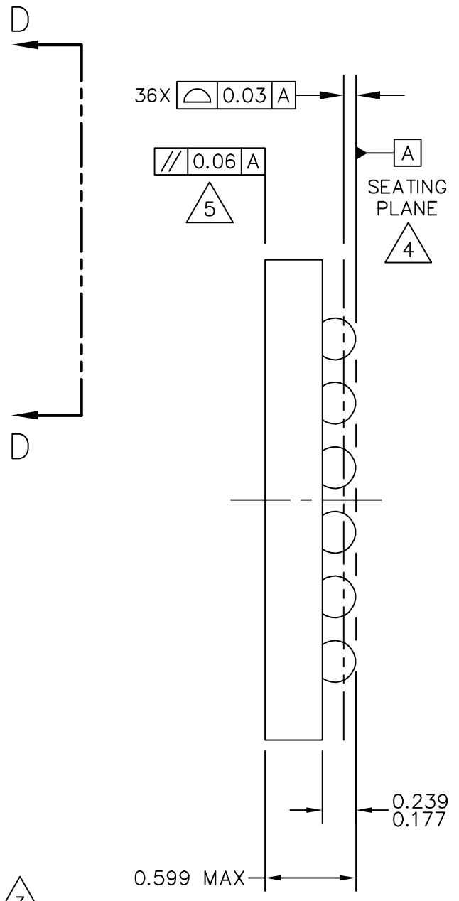
VIEW D-D
