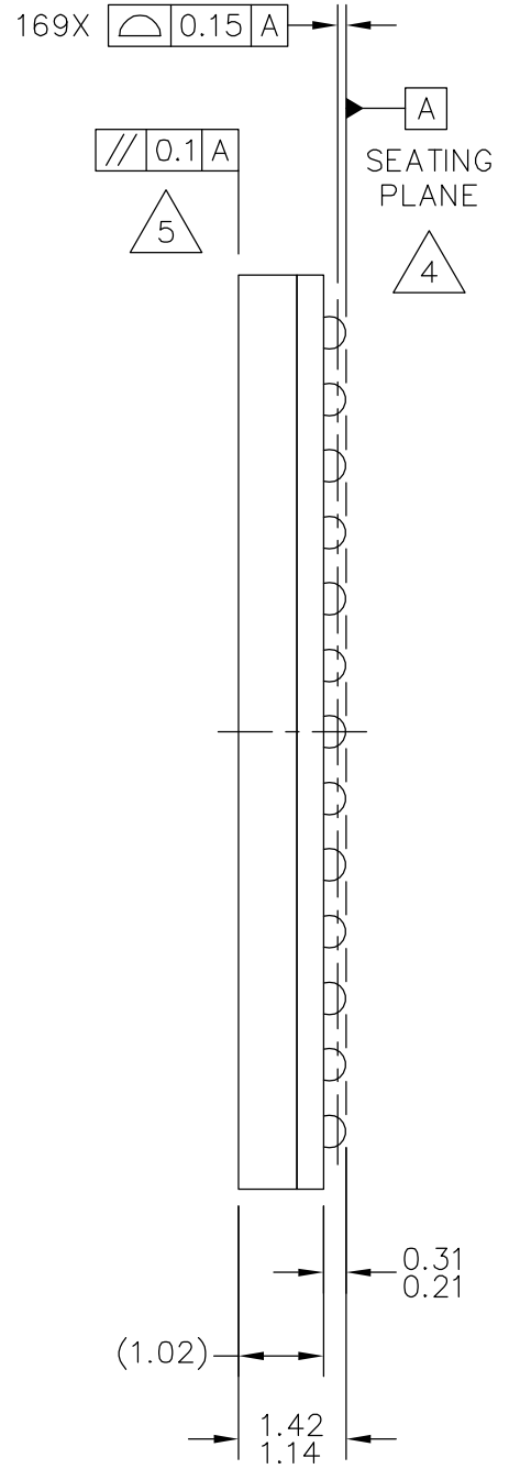
SIDE VIEW
