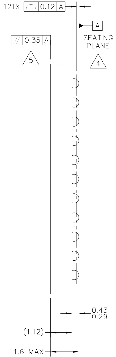
SIDE VIEW
