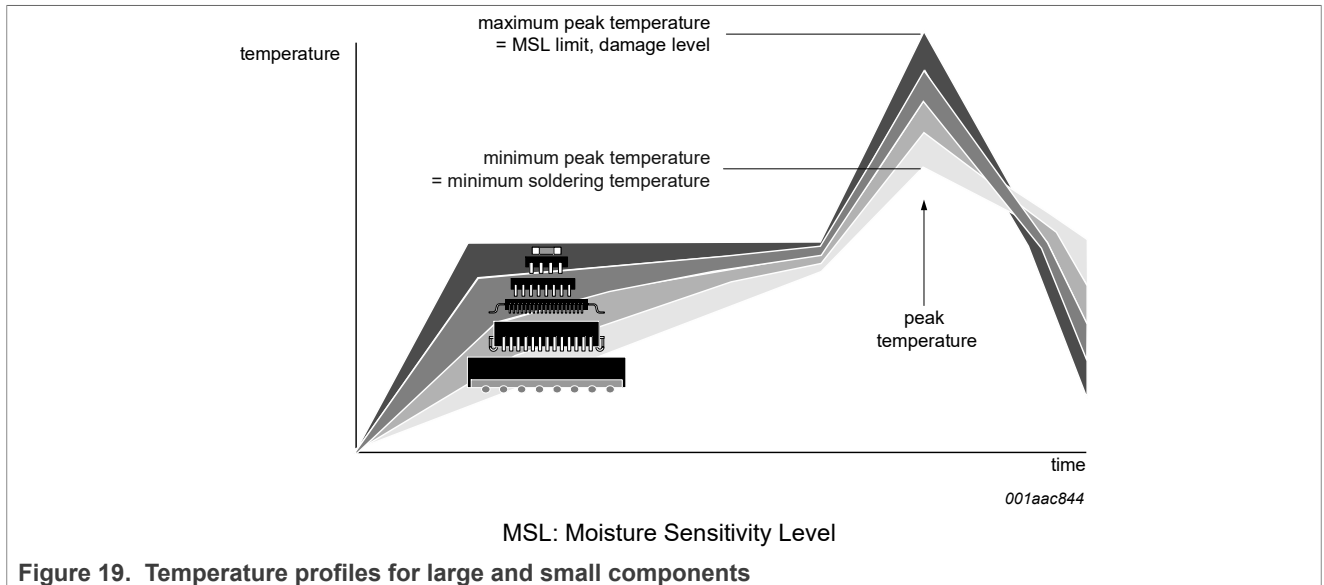
Figure 19. Temperature profiles for large and small components
