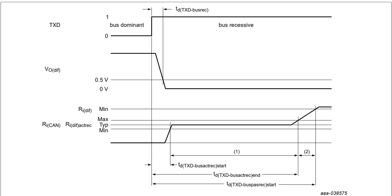
Figure 14. Transmitter impedance and timing diagram for dominant-to-passive recessive transition according to ISO 11898-2:2024 parameter set C
