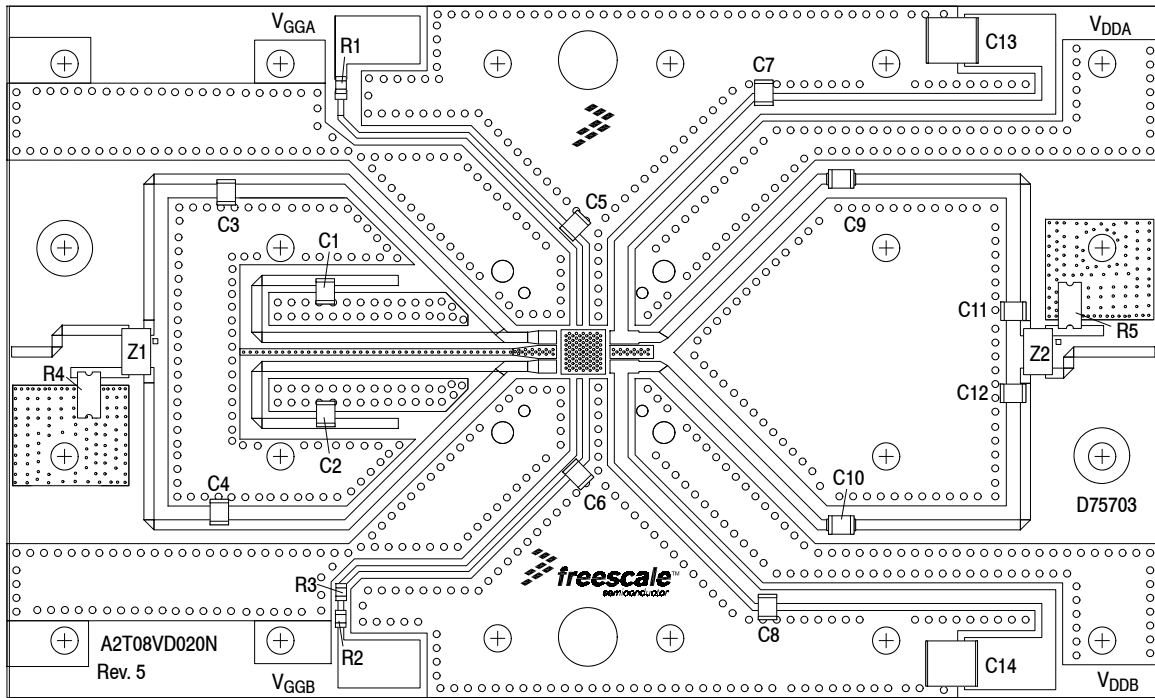
Figure 3. A2T08VD021NT1 Test Circuit Component Layout
