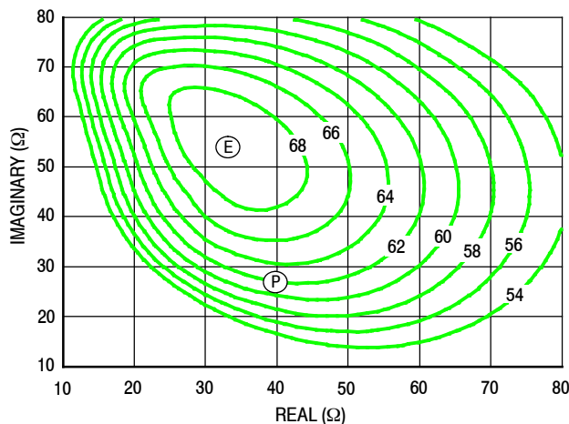
Figure 22. P1dB Load Pull Efficiency Contours (%)
