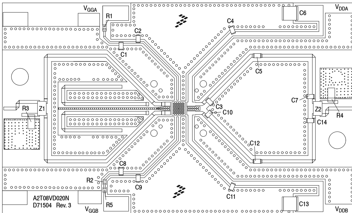
Figure 17. A2T08VD021NT1 Test Circuit Component Layout — 728–768 MHz
