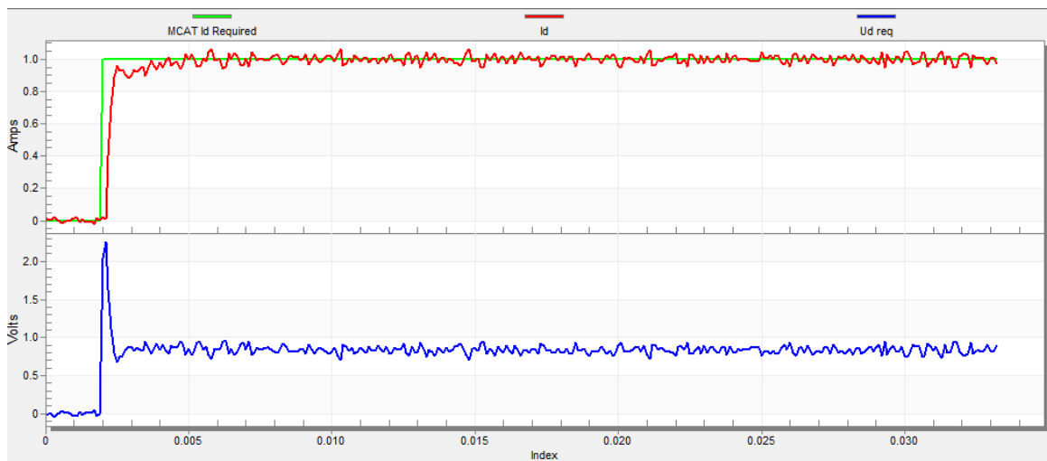
Figure 26. Optimal step response of Id current controller
