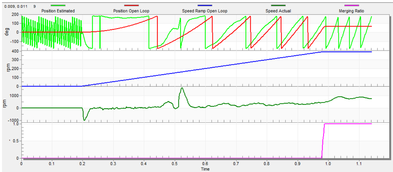
Figure 29. Motor startup
