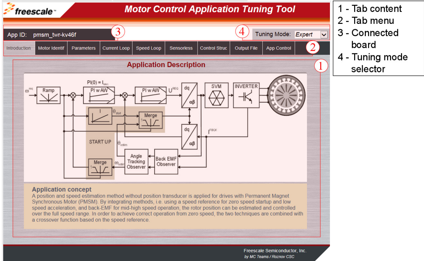
Figure 10. MCAT layout
